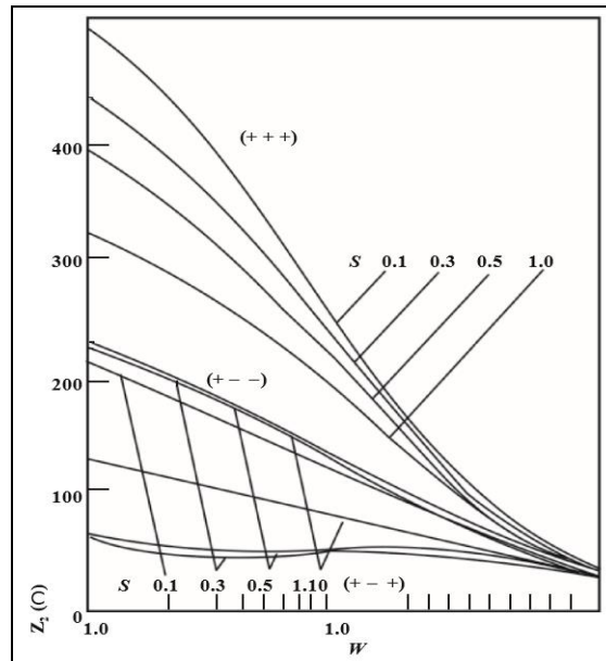
Fig 4: Characteristic Impedance of the Middle Conductor Z_2 ( W = 1.0 ; T = 0.1 )
