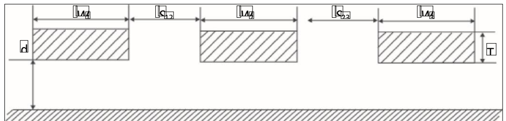
Fig 1: Cross Section of Three Conductor Strip Line
