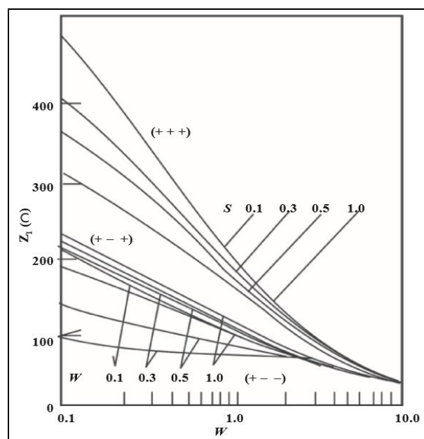
Fig 3: Characteristic Impedance of the End Conductor Z_1 ( W = 1.0 ; T = 0.1 )
