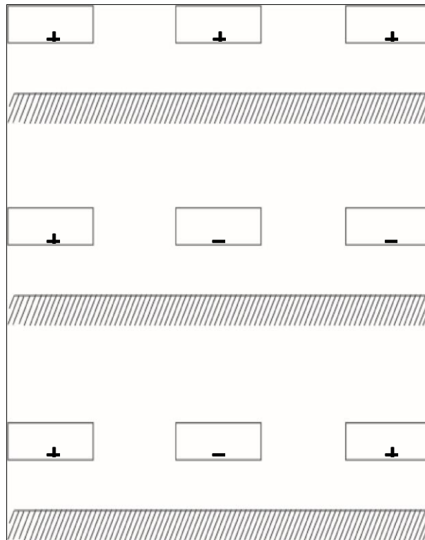
Fig 2: Three Kinds of Excitation of Three Conductor Strip Line
