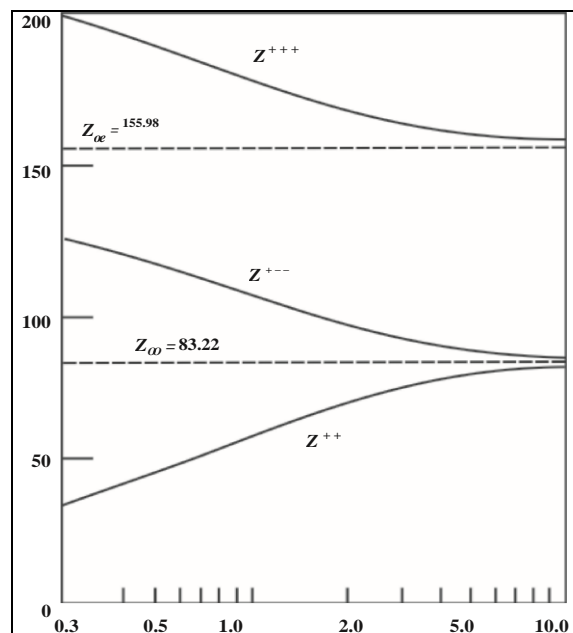
Fig 5: The Influence of Distance S_{23} on the Characteristic Impedance Z_2
